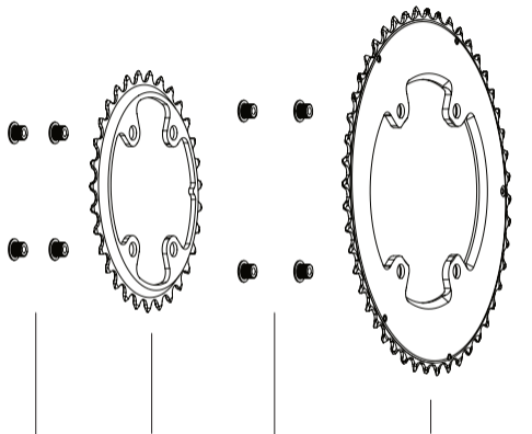
ROTOR Inner Chaining
